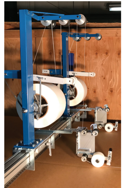
Dry End Tape Applicator shown on a support stand.
